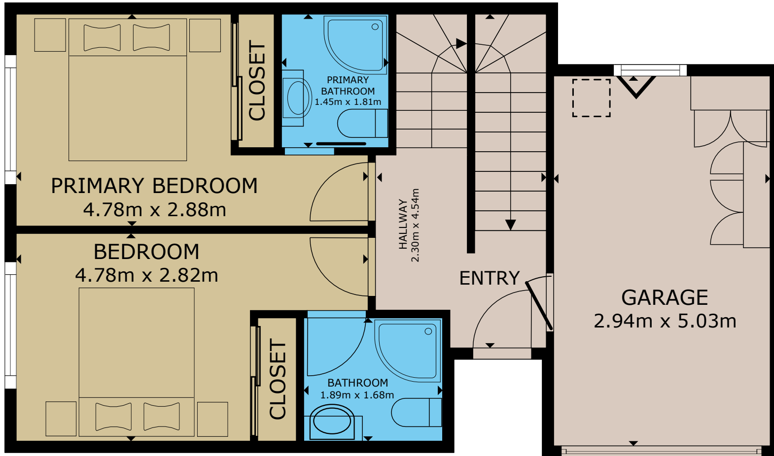
FLOOR 2
