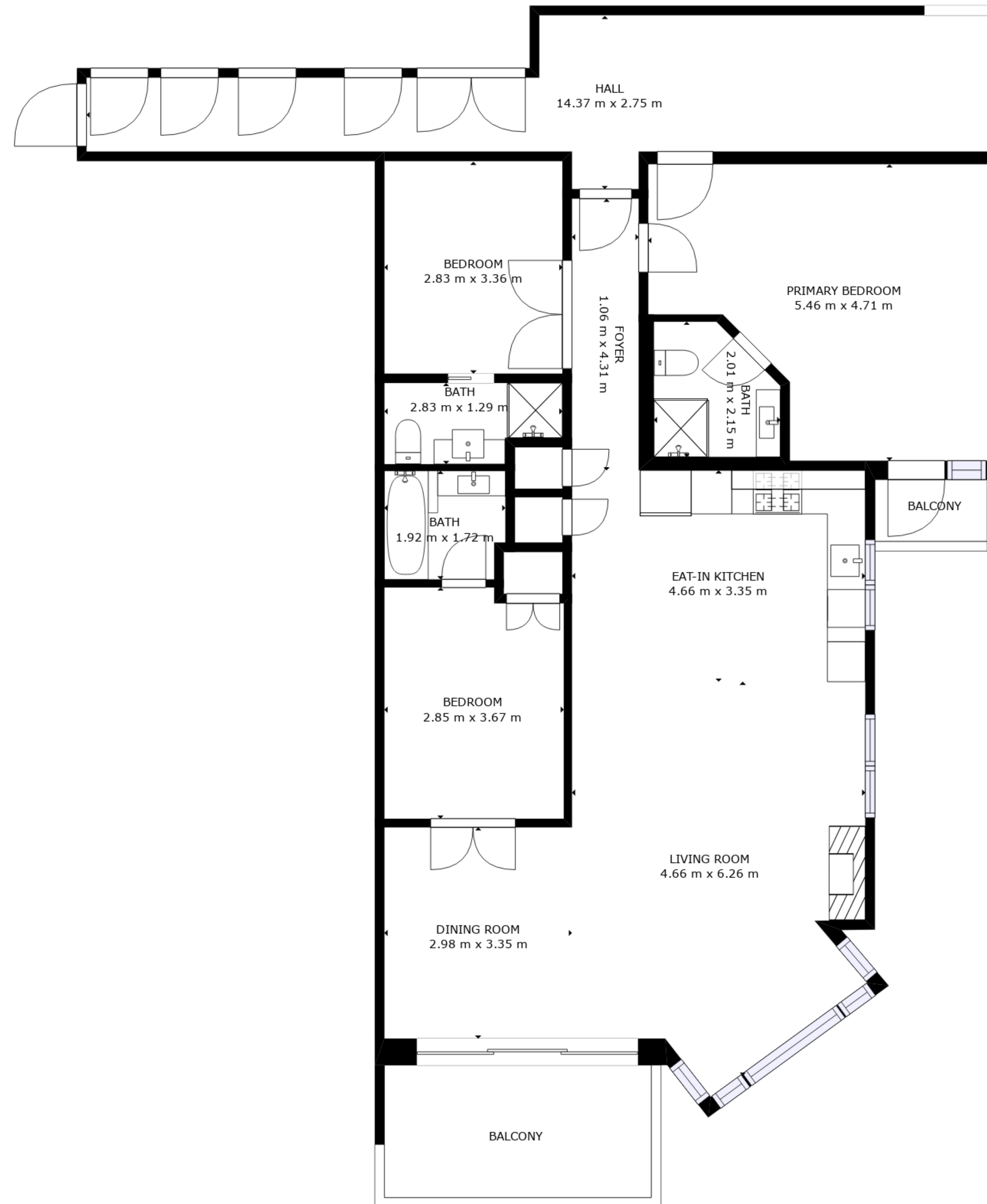
FLOOR 1
