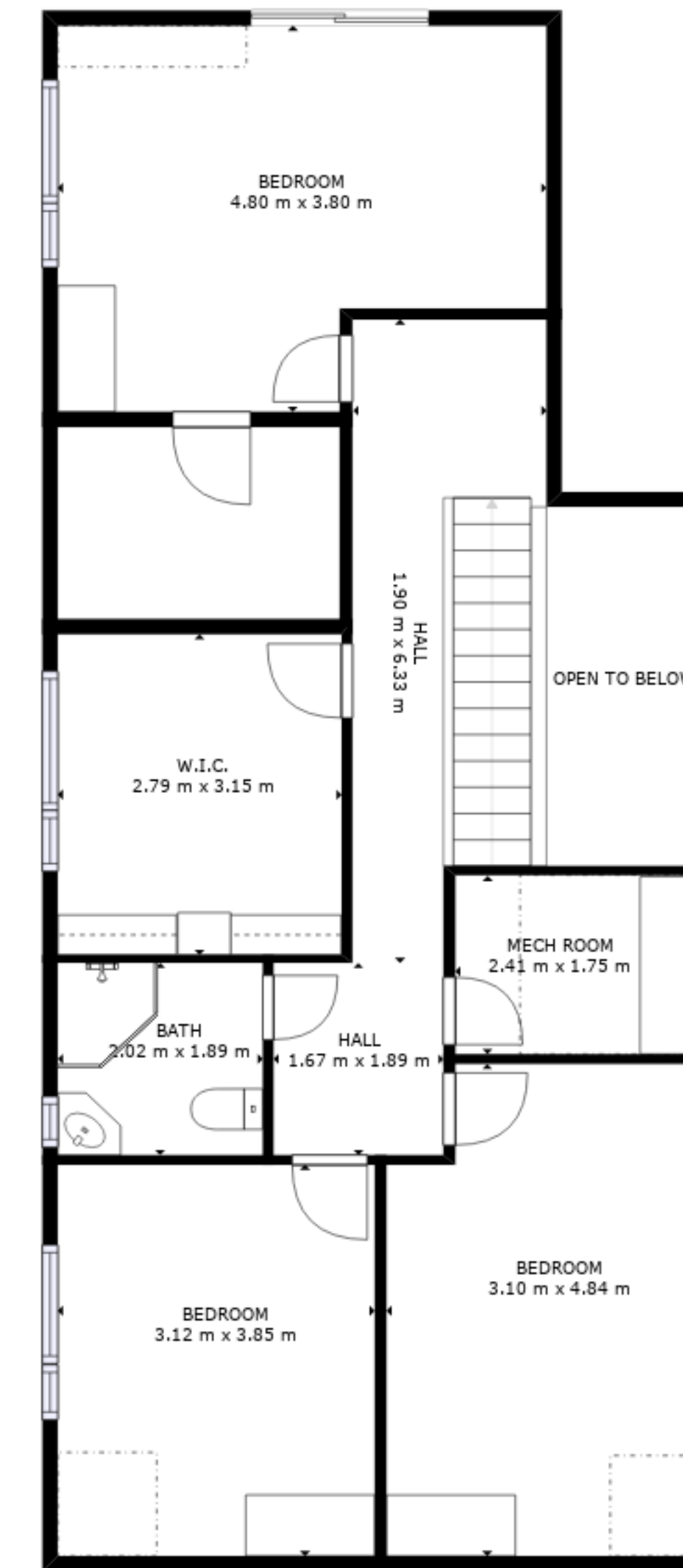
FLOOR 2
